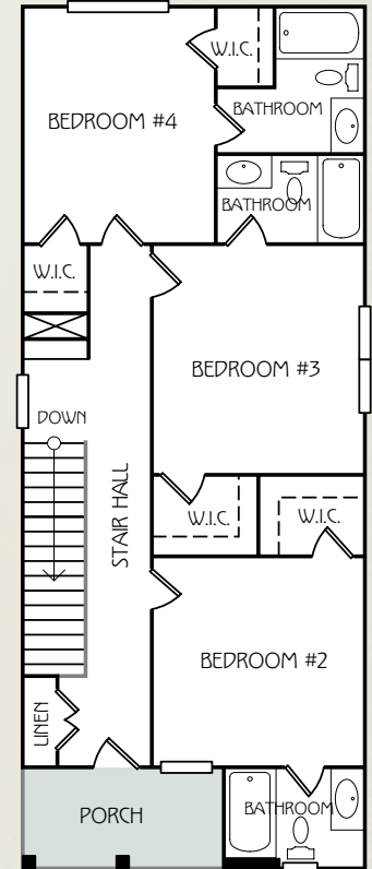
2ND FLOOR
